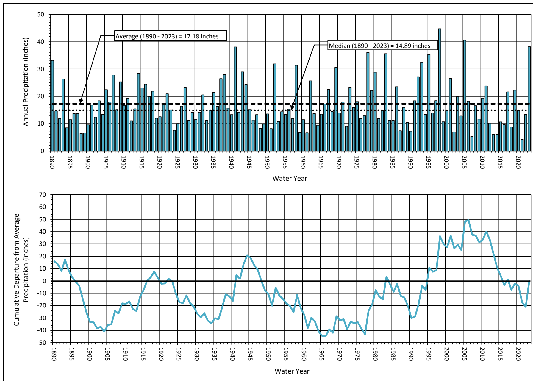
Figure 2. Annual Precipitation at Santa Paula and Cumulative Departure from Average, WYs 1890 through 2023
