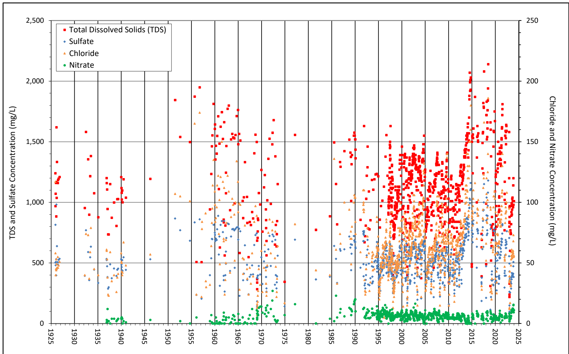
Figure 8. Concentrations of Selected Major Surface Water Quality Parameters in the Santa Clara River at Freeman Diversion, CYs 1925 through 2023
