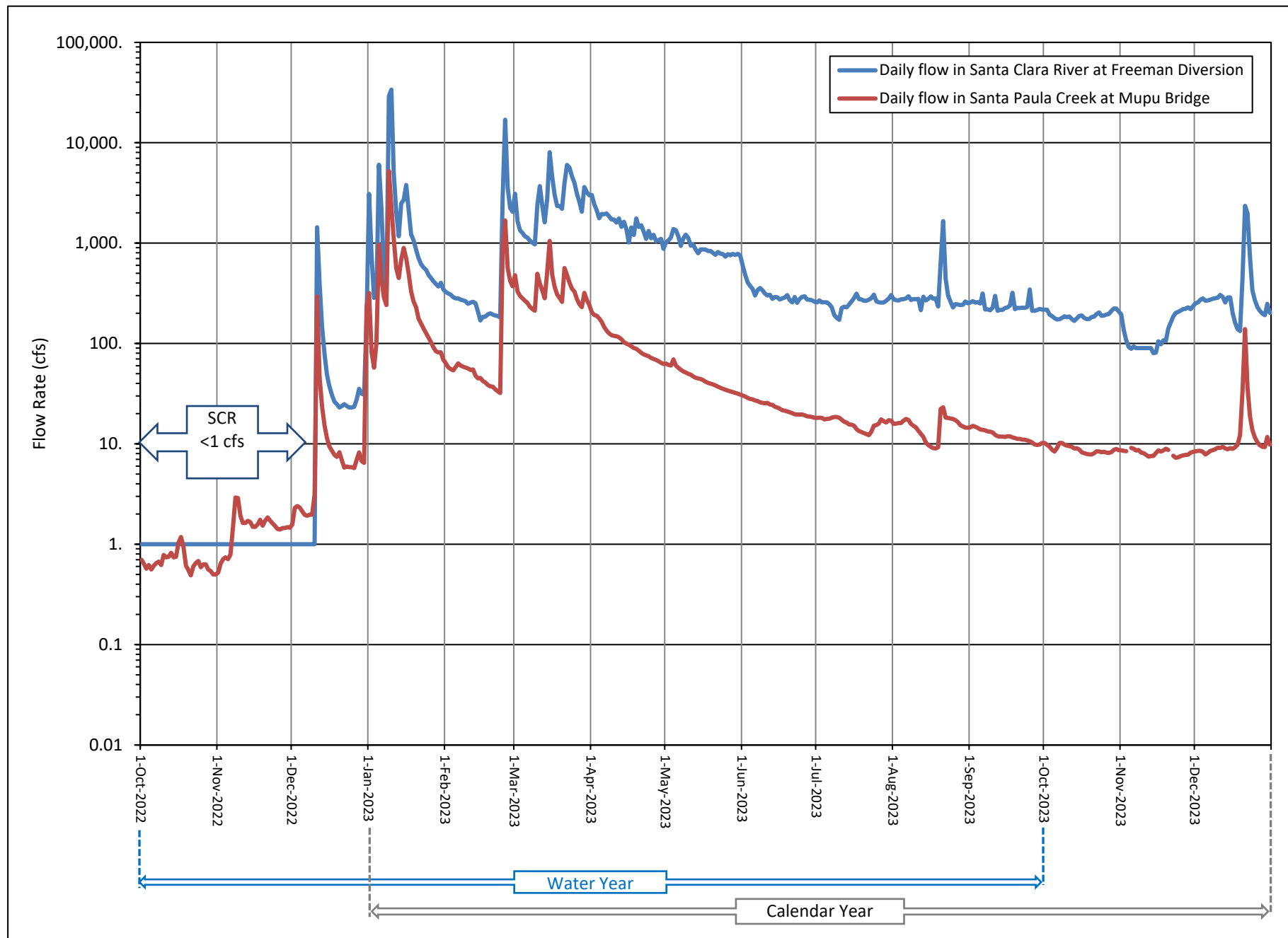
Figure 7. Daily Streamflow in Santa Paula Creek and Santa Clara River, WY and CY 2023
