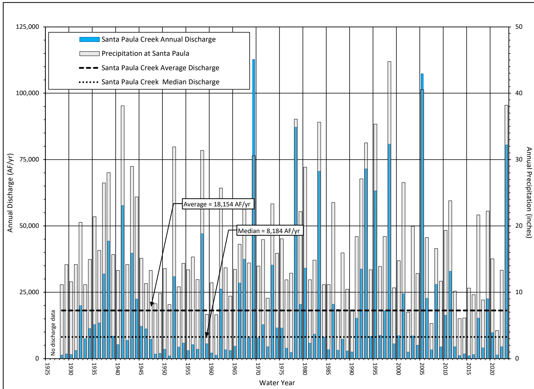
Figure 6. Annual Discharge of Santa Paula Creek Near Santa Paula, WYs 1928 through 2023
