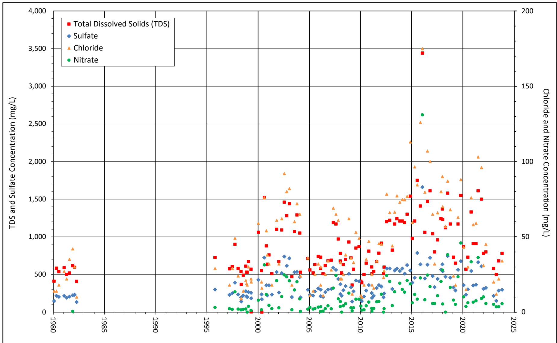
Figure 9. Concentrations of Selected Major Surface Water Quality Parameters in Santa Paula Creek Near Santa Paula, CYs 1980 through 2023
