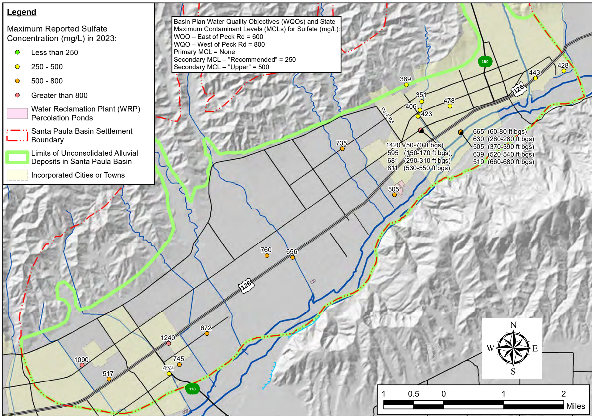
Figure 20. Maximum Reported Sulfate Concentrations in Groundwater, CY 2023
