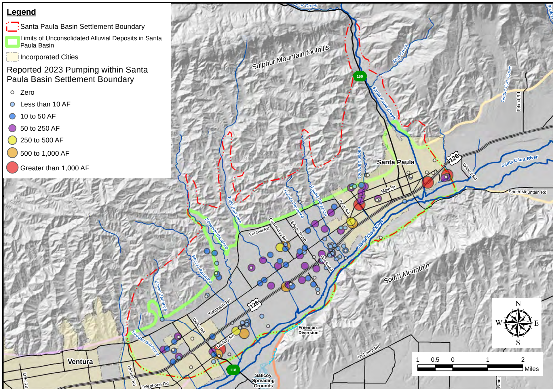
Figure 12. Santa Paula Basin Groundwater Extractions by Well, CY 2023
