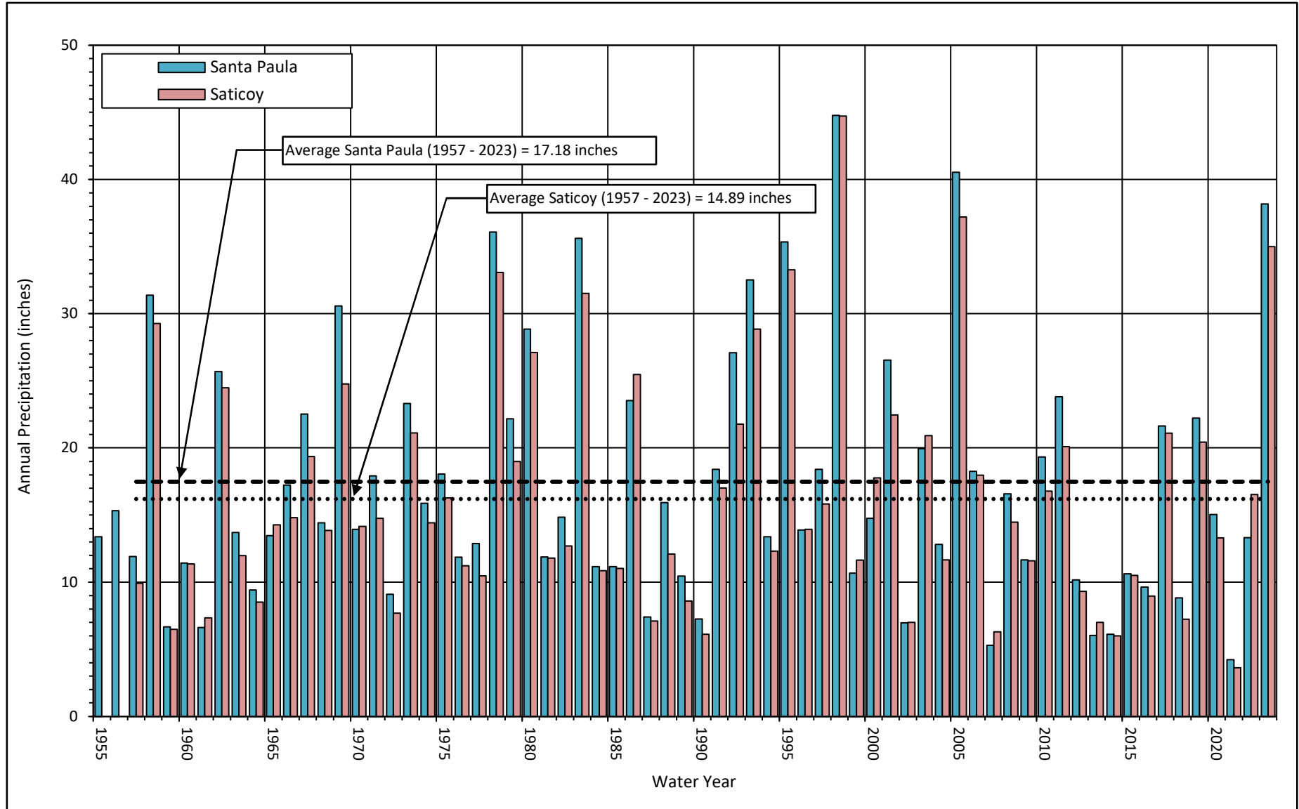
Figure 3. Annual Precipitation at Saticoy and Santa Paula, WYs 1955 through 2023
