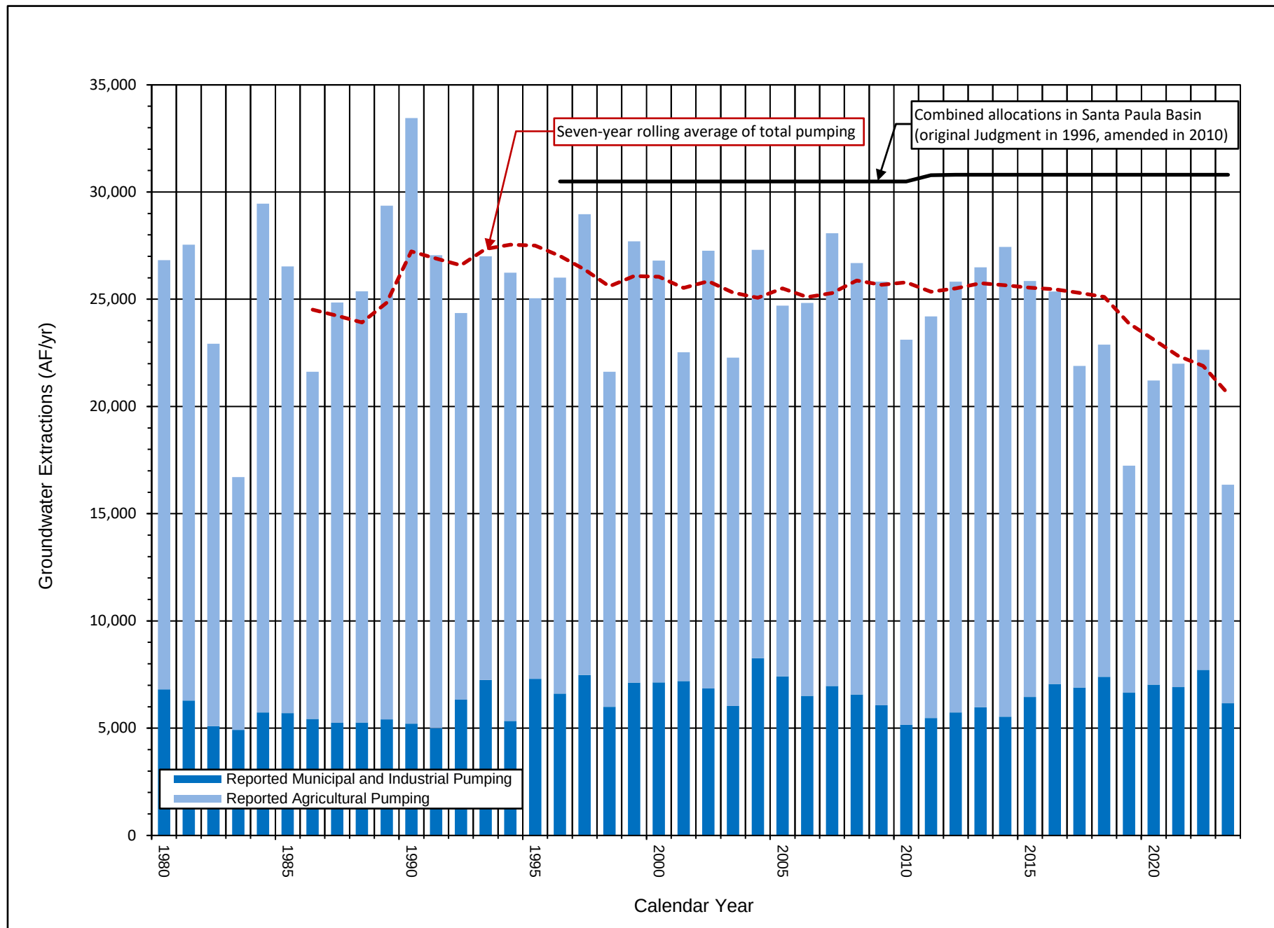
Figure 10. Historical Annual Groundwater Extractions from Santa Paula Basin, CYs 1980 through 2023
