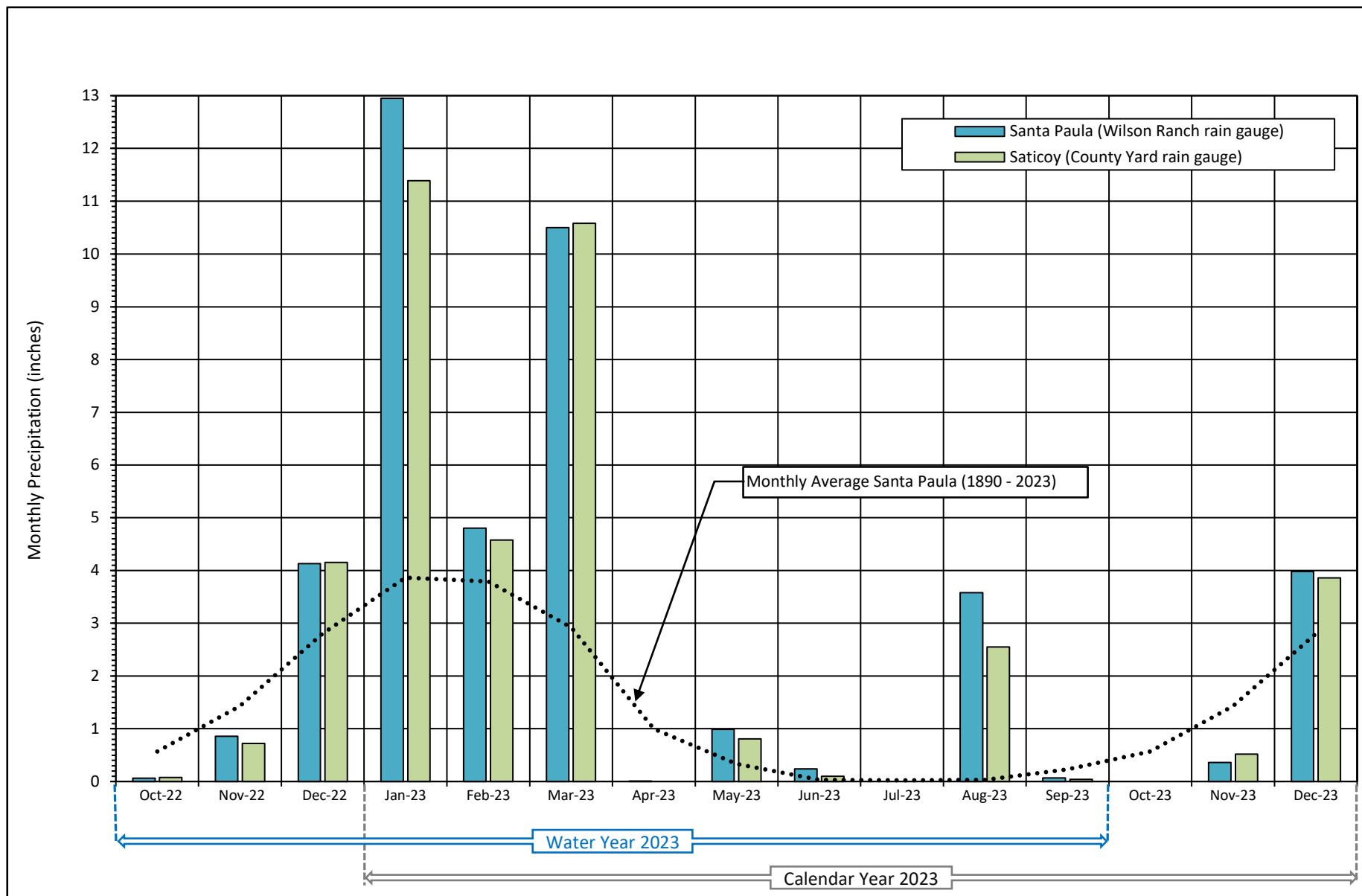
Figure 4. Monthly Precipitation in Santa Paula Basin, WY and CY 2023
