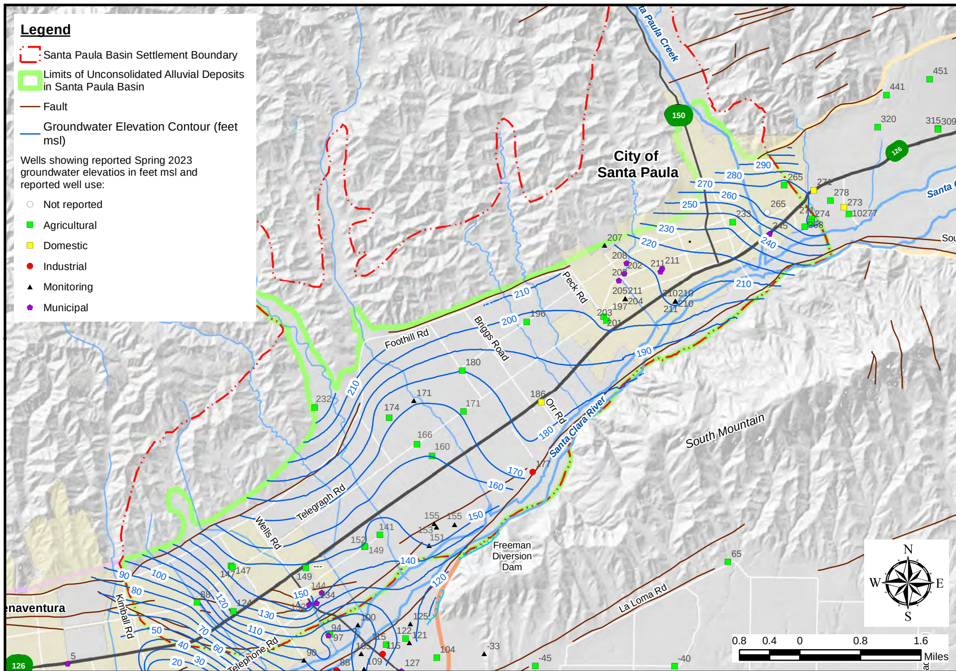
Figure 14. Santa Paula Basin Groundwater Elevation Contours, Spring 2023
