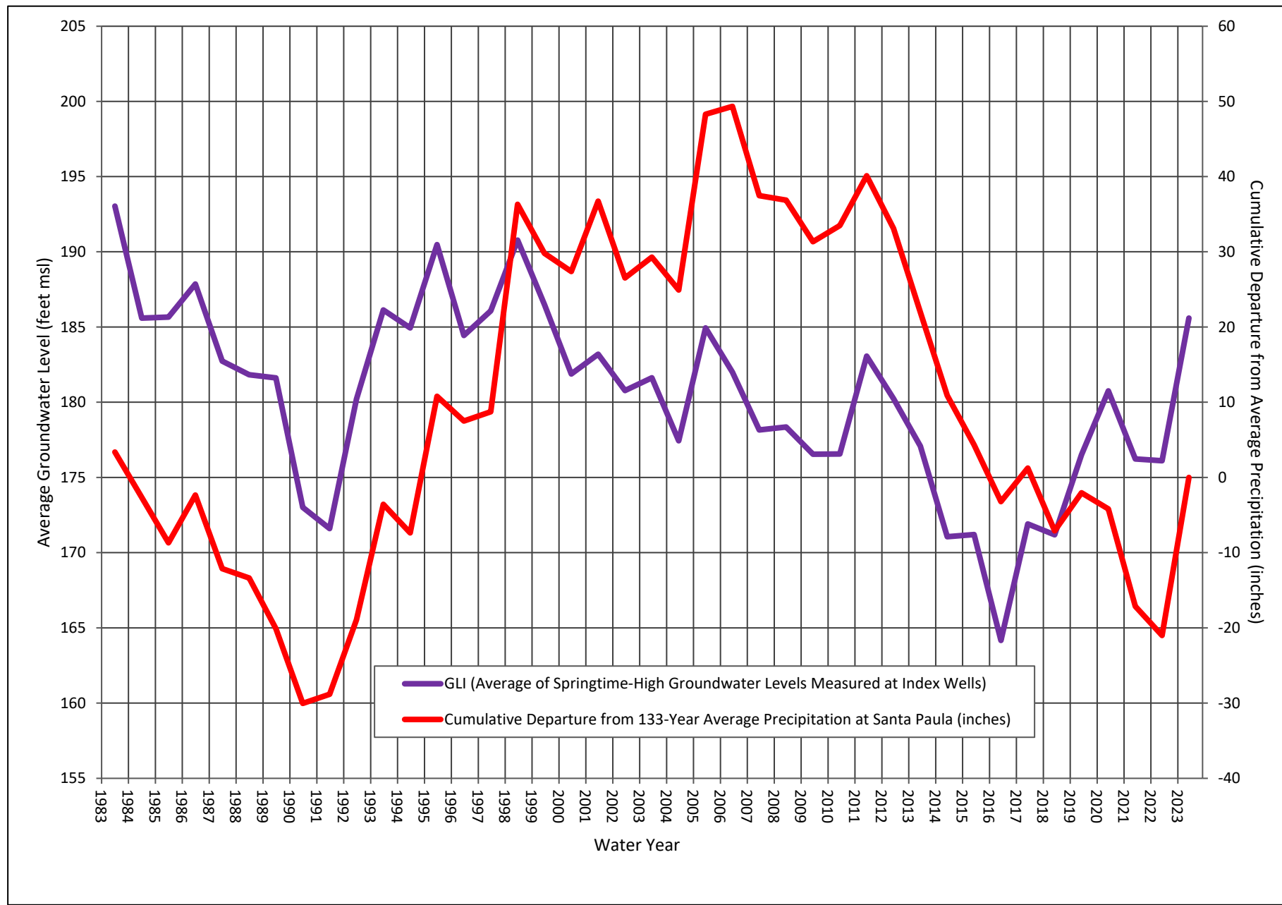
Figure 16. Groundwater Level Index and Cumulative Departure from Average Precipitation in Santa Paula Basin, WYs 1983 through 2023
