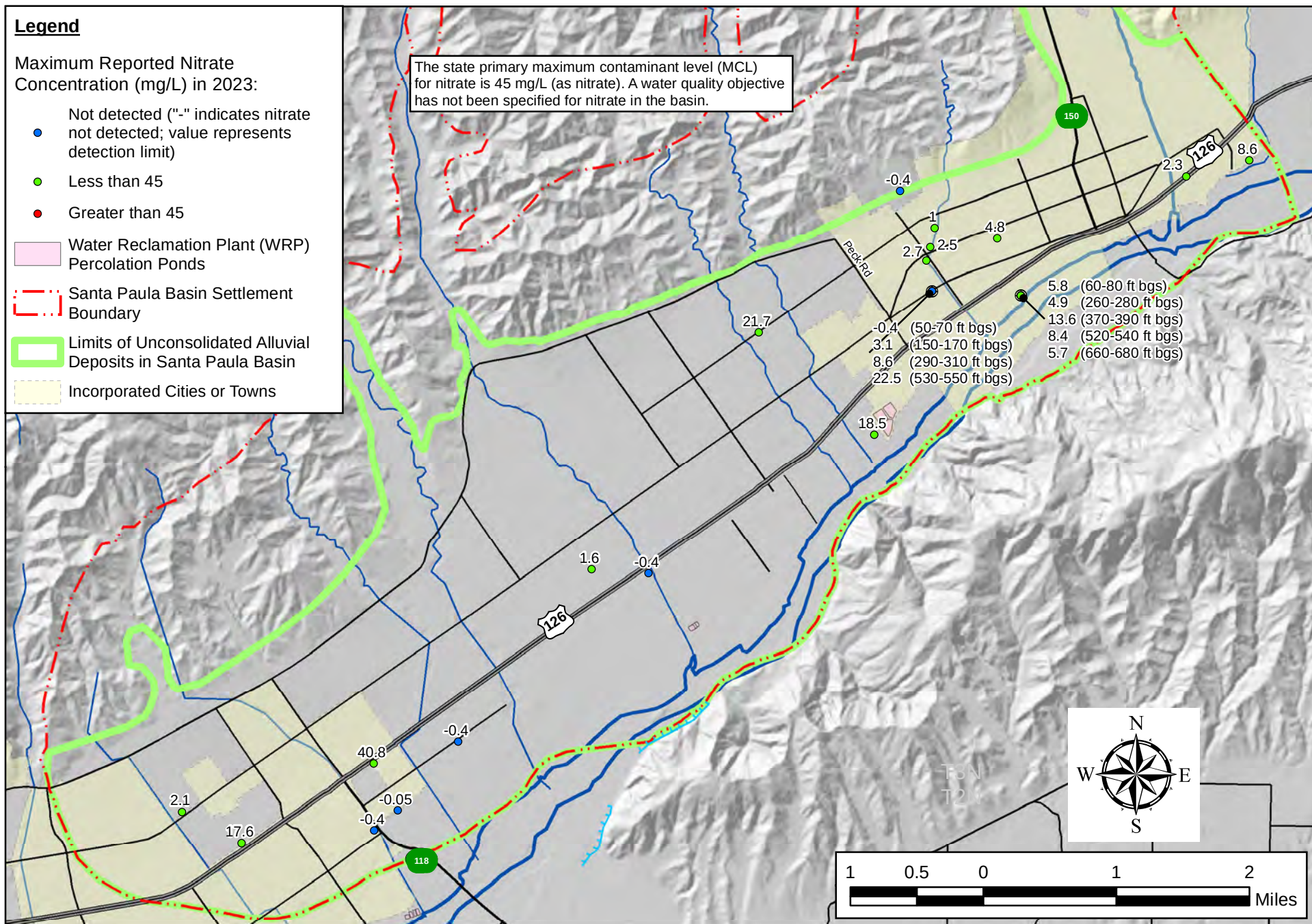
Figure 18. Maximum Reported Nitrate Concentrations in Groundwater, CY 2023
