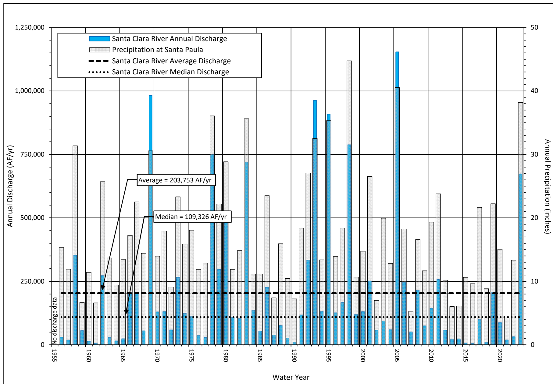
Figure 5. Annual Discharge of Santa Clara River at the Freeman Diversion, WYs 1956 through 2023
