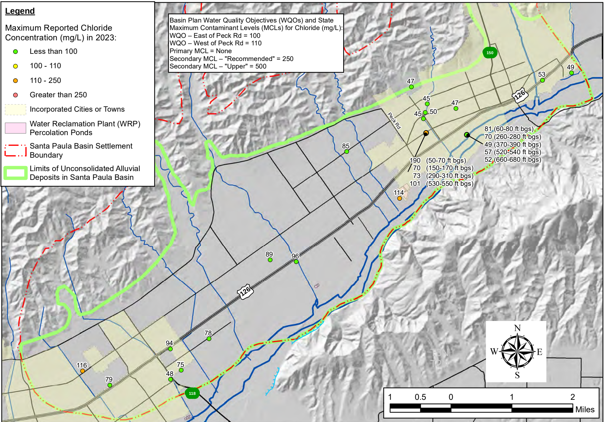
Figure 19. Maximum Reported Chloride Concentrations in Groundwater, CY 2023
