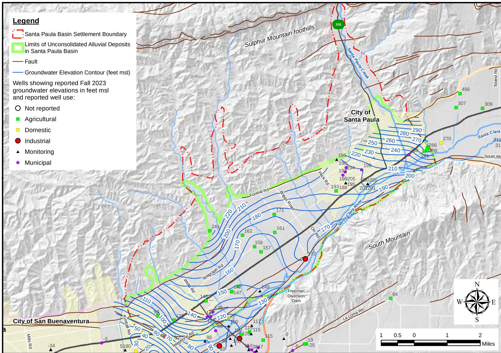
Figure 15. Santa Paula Basin Groundwater Elevation Contours, Fall 2023
