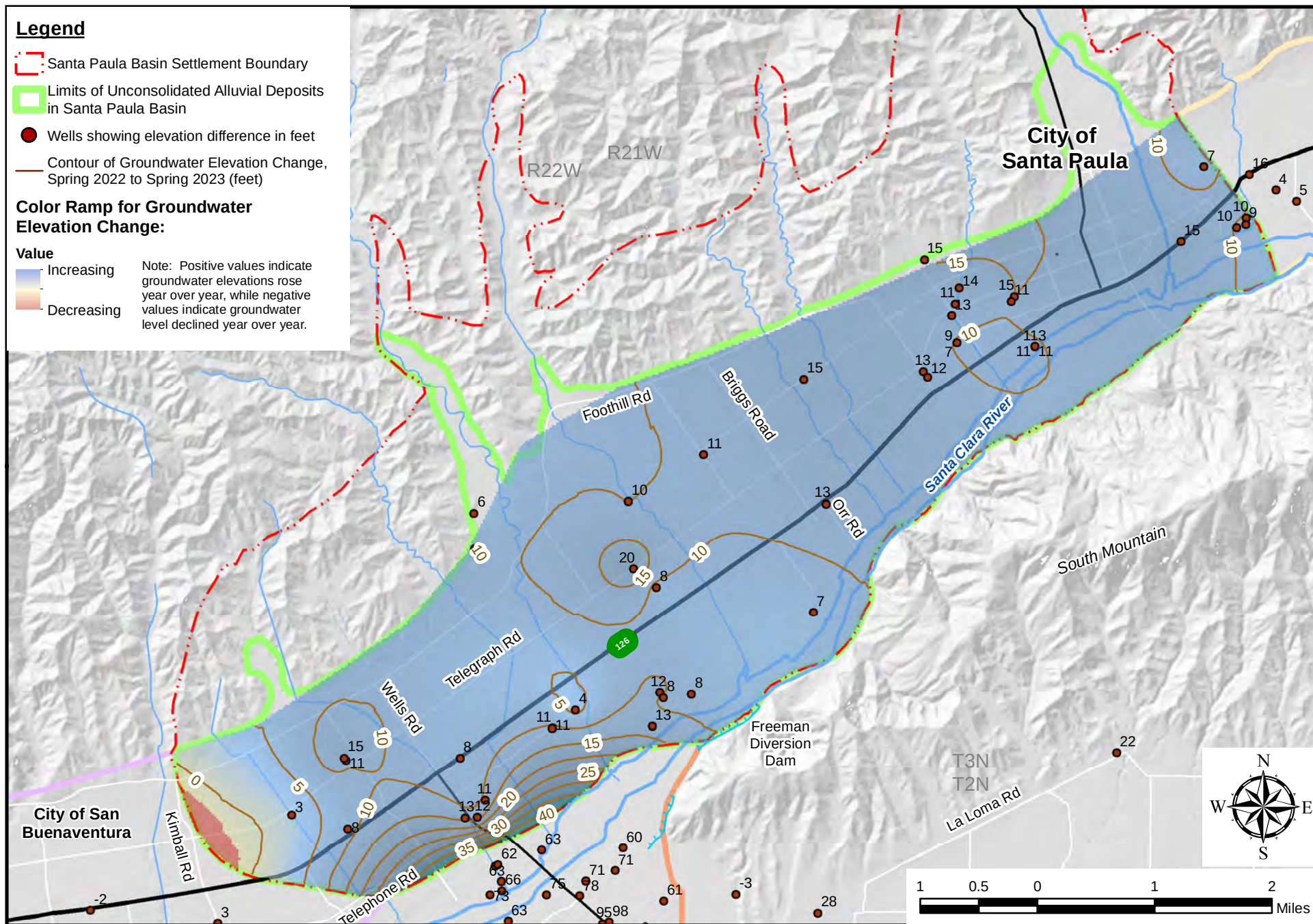
Figure 17. Change in Groundwater Elevation in Unconsolidated Alluvial Deposits of Santa Paula Basin, Spring 2022 to Spring 2023
